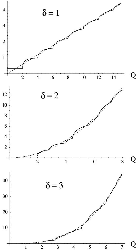
FIG. 1. \mathcal{I}\Pi^{(\delta)}(Q) as compared with the asymptotic value ( \delta = 1, 2, 3 ). Q is given in units of M_c .
